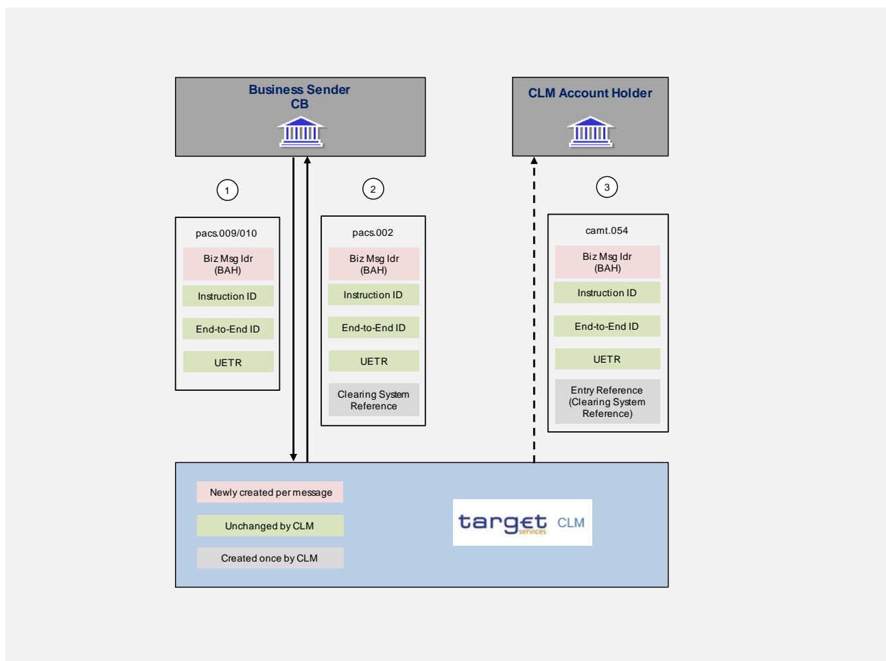
Figure 91 - Message References
