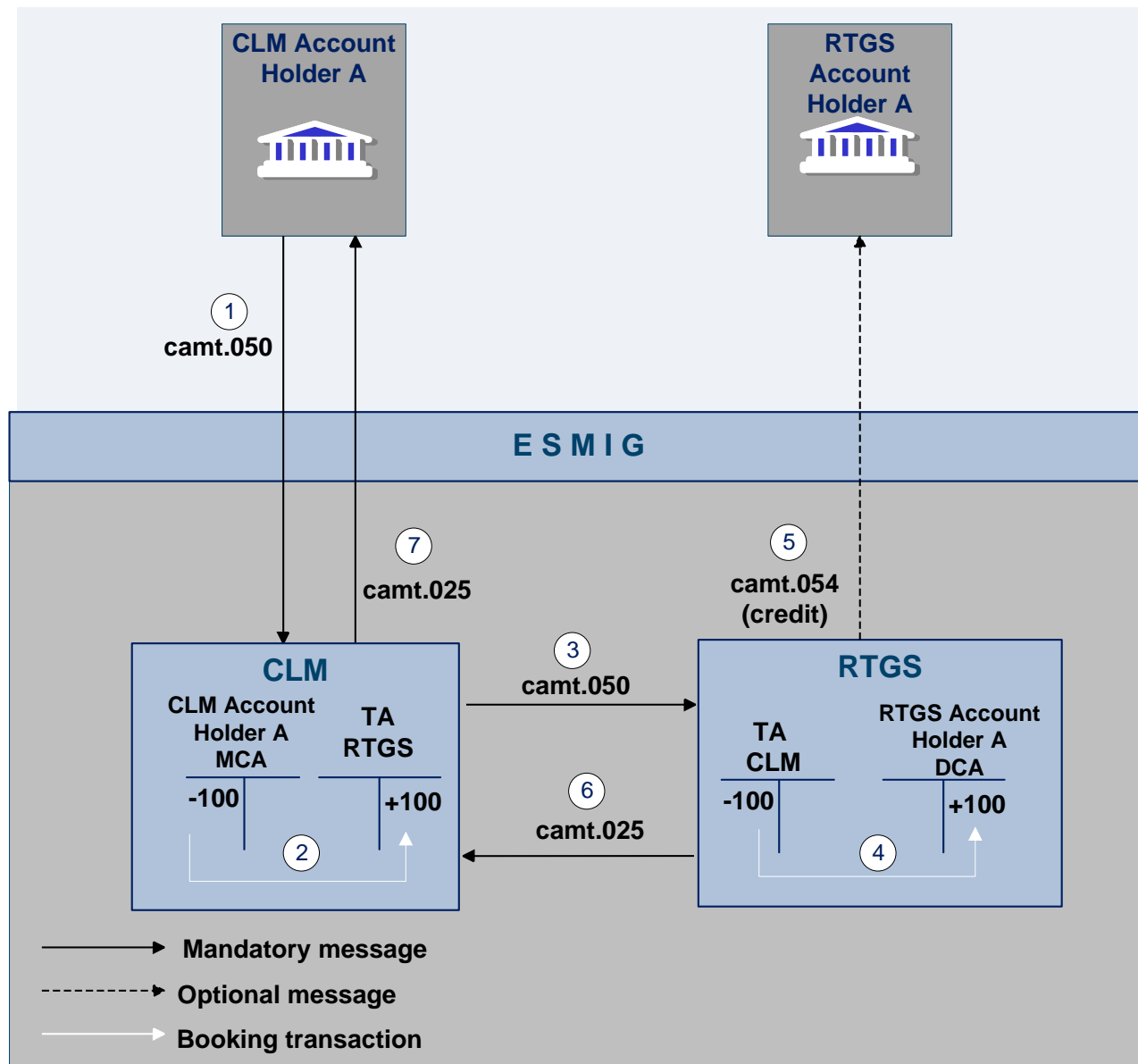
Figure 25 - Example camt.050 inter-service liquidity transfer from MCA to RTGS DCA
